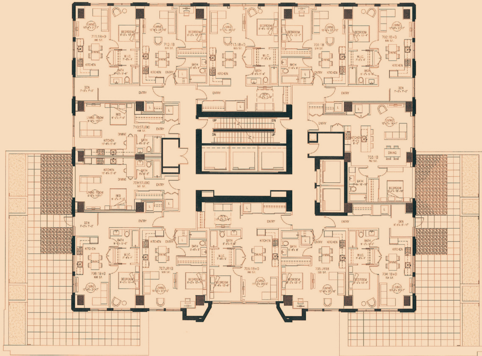
6th Ave podium typical floor plan level 7
